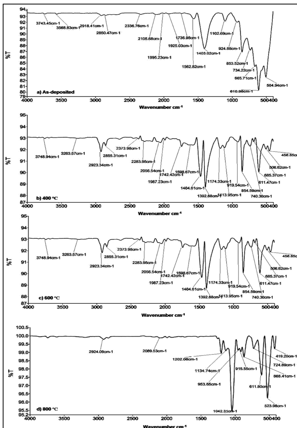
Fig. 7. FTIR spectrum of \text{BaTiO}_3 thin film at (a) As-deposited, (b) 400 °C, (c) 600 °C and (d) 800 °C annealing temperatures
