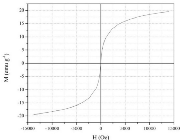
Fig. 4. Hysterersis loop of sample GC.
